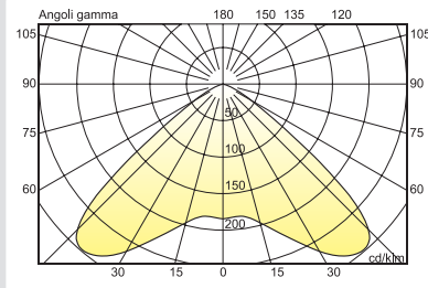
VOGUE RP 150W MC
