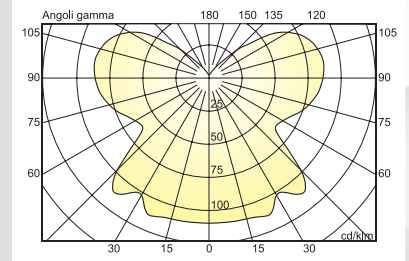
VOGUE GFA/40 150W ME
