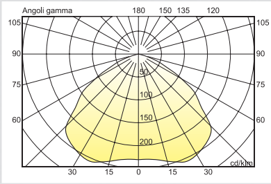
VOGUE 42W FSM
