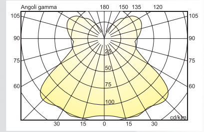
VOGUE GOA/30 150W ME
